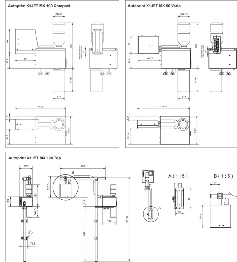
Autoprint X1JET MX 100 Compact All the controls are housed in this compact system.
