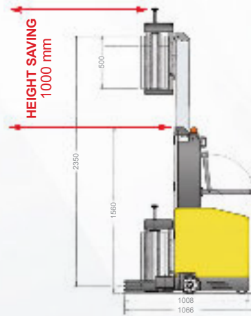
TELESCOPIC MAST
